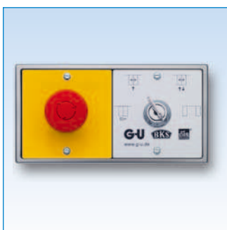
Combined switch EMERGENCY-OFF/Function selection, flush mounted standard white Article number: A-8002290
